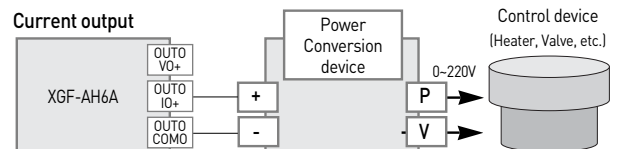
Current output
