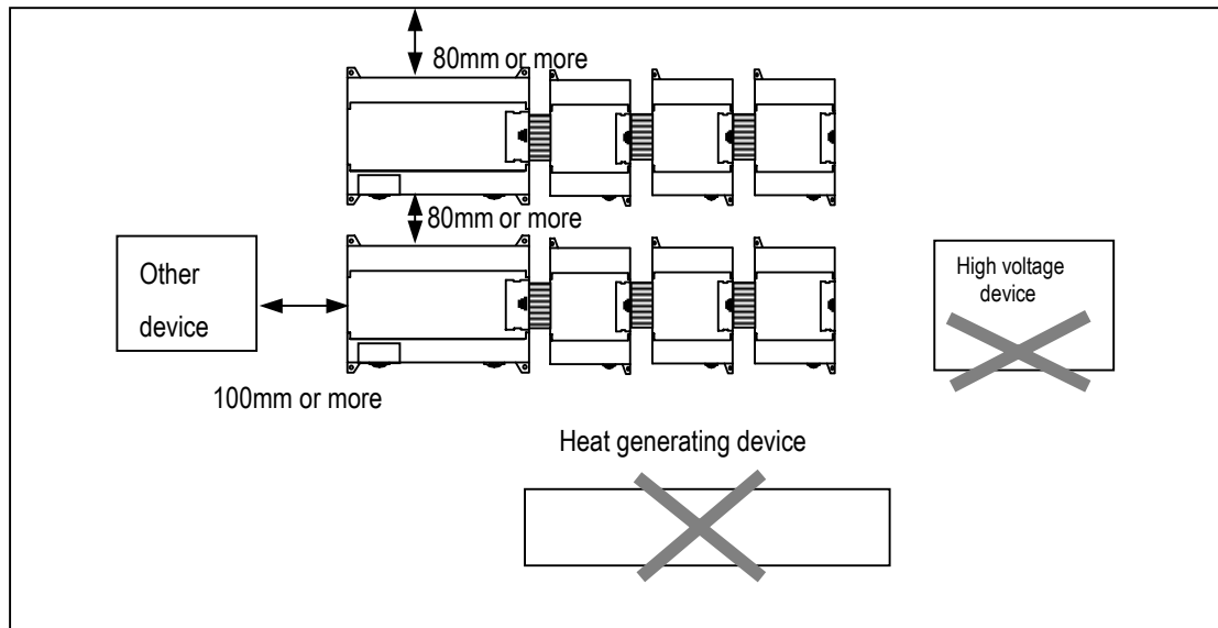
[ Fig 9.2 ] PLC mounting
