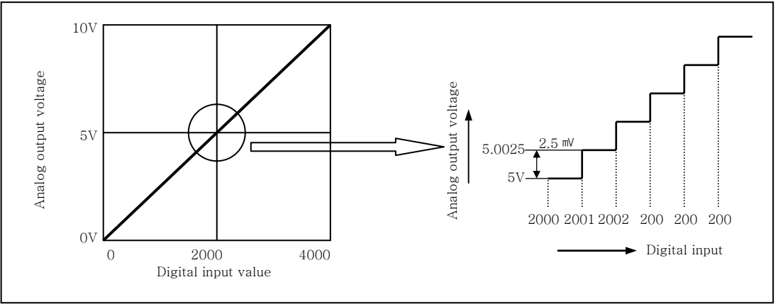
D/A conversion characteristic (voltage output)
