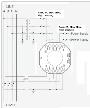
< PIC 5 3P 4W connection with 3PT >
