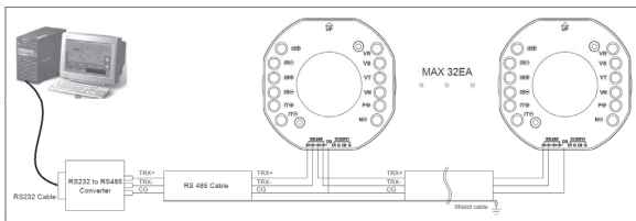
< PIG13 RS-485 Communication Wiring Connection >
