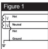
SPLIT 2 Hots, 1 Neu, 1 Gmd
