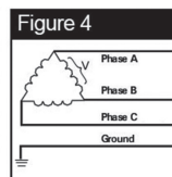
DELTA & HRG WYE 3 Hots, 1 Gmd
