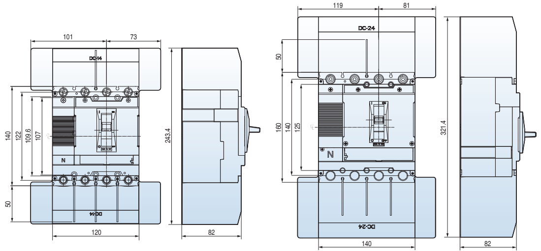
4P (L-type)
