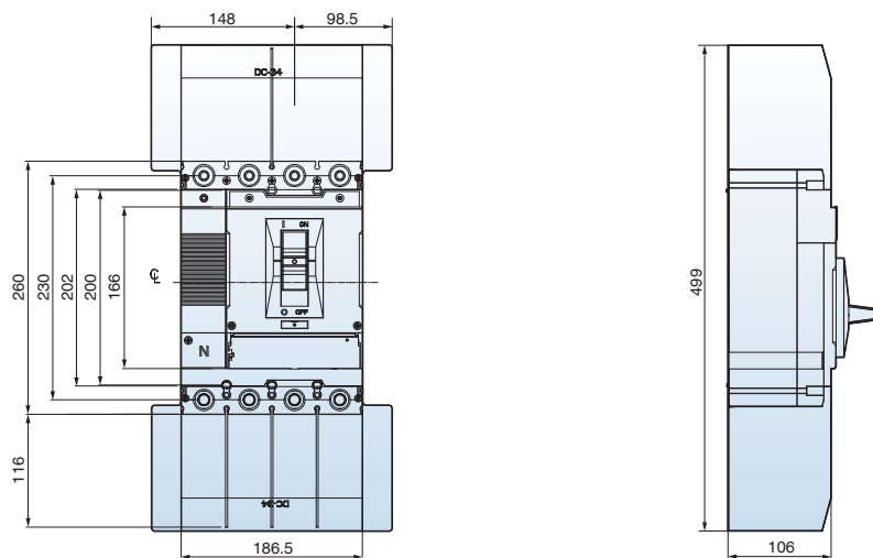
4P (L-type)
