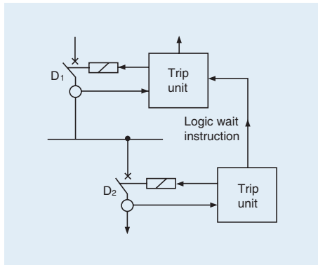
(c) Zone selective interlocking
