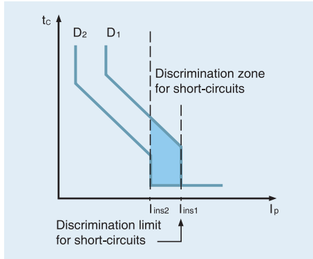
(a) Current discrimination
