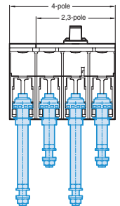
Round type
