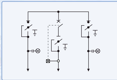
LCL ( 2L1C )
